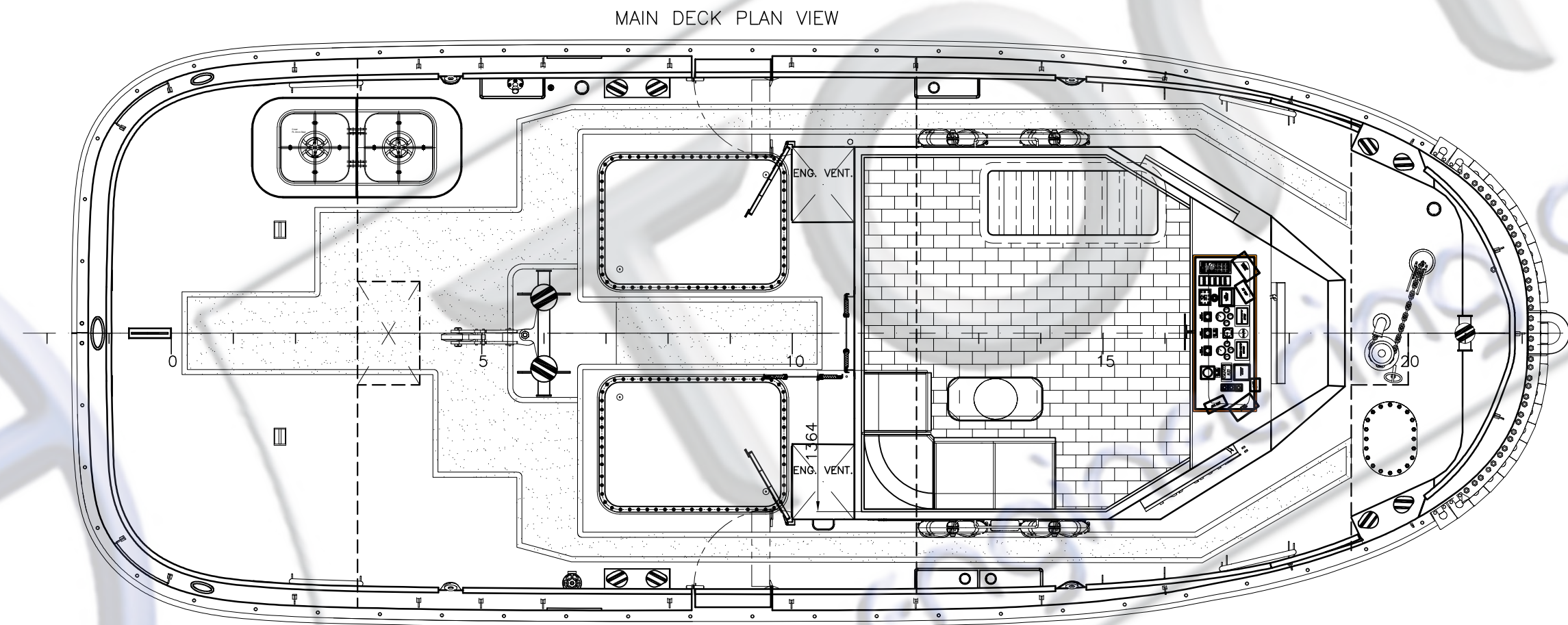
MAIN DECK PLAN VIEW
